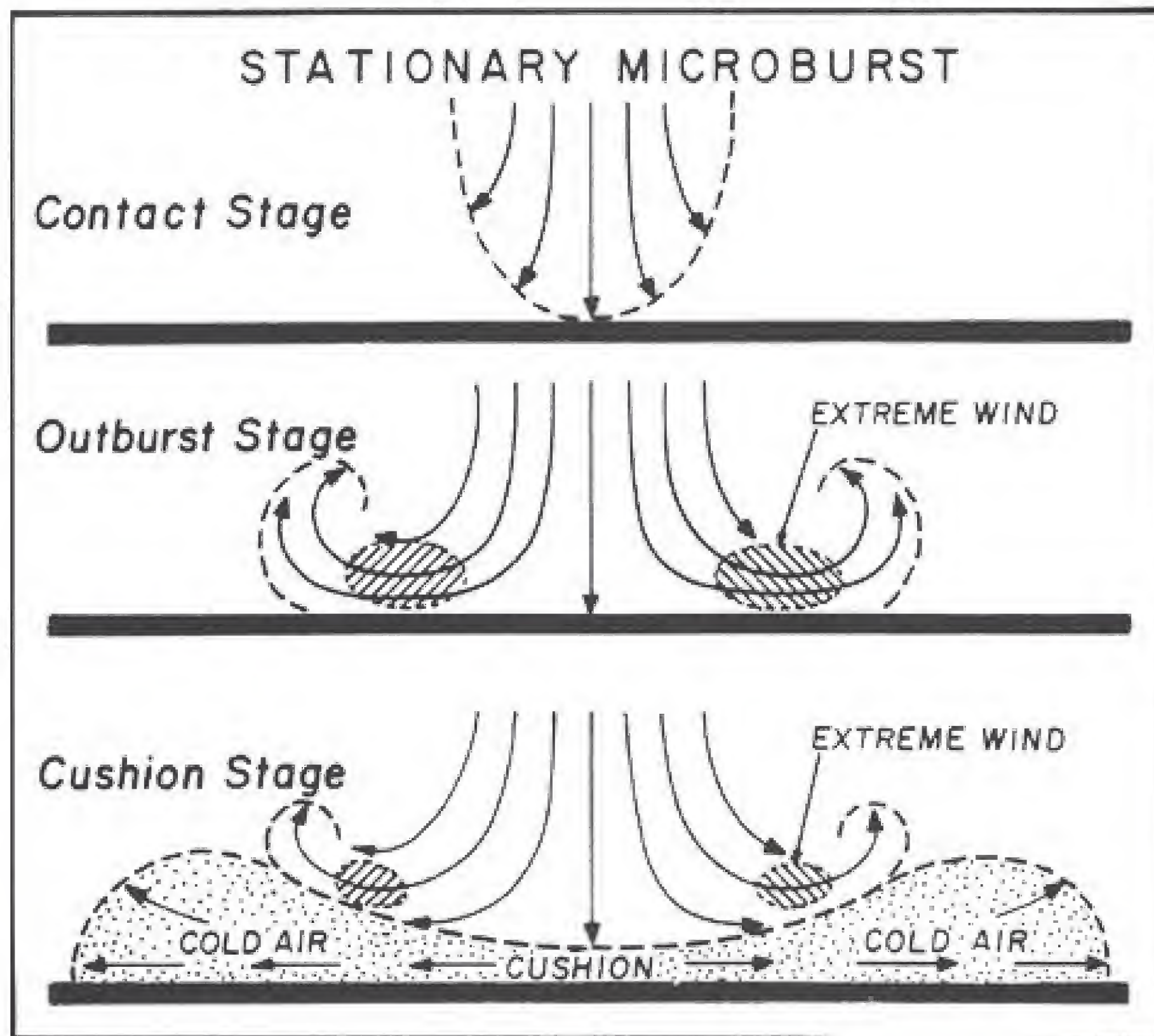
Figure 25. Life cycle of a microburst.
